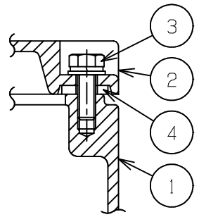
“A”部詳細 (1/3)
