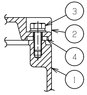
“A”部詳細(1/3)
